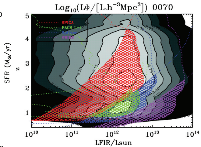
Figure 16 - A plot of the FIR Luminosity density (i.e. luminosity-weighted luminosity function) as a function of FIR luminosity and redshift (greyscale and contours). This illustrates the galaxies and epochs that contribute most to the star-formation history of the Universe (in the model of Lagache et al. 74 ). The ability of 70 \mu\text{m} surveys to probe this function is indicated by colour hatching: SPICA (1000sq. arcmin 50 \mu\text{Jy} red); Spitzer (Deep surveys -- Blue and SWIRE--Magenta). Herschel GT surveys cannot constrain this function at 70 \mu\text{m} , while the power of the 110 \mu\text{m} surveys are shown (green). Herschel and Spitzer sample the z\sim 1 peak: only SPICA can probe the z\sim 2.5 peak.
