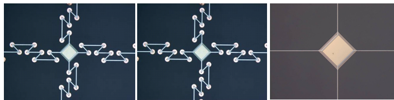
Figure 21 – Various prototype ESI detectors tested at SRON. The detector on the right achieved a performance close to the ESI goal.
