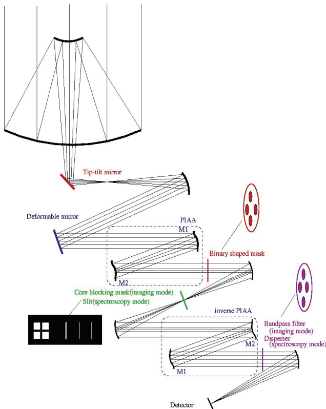
Figure 23 - Schematic optical layout of the Coronagraph and key specifications
