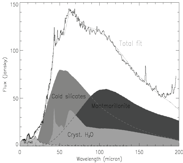
Figure 6: The ISO spectrum of the young star HD 142527 22 showing the model components including the crystalline water ice features. Water ice can only be directly detected at these temperatures through the 44 and 63 \mu\text{m} emission features. SPICA will be able to take the equivalent spectra of objects at flux levels of \sim 1 mJy in one hour.
