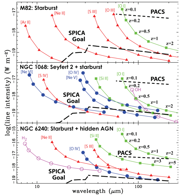
Figure 12 - A plot of intensity vs. redshift of a selection of the key MIR/FIR emission lines visible with SPICA in three archetypical objects: M82 ( L_{\text{FIR}} \sim 4 \times 10^{10} L_{\odot} ), NGC1068 ( L_{\text{FIR}} \sim 2 \times 10^{11} L_{\odot} ) and NGC6240 ( L_{\text{FIR}} \sim 7 \times 10^{11} L_{\odot} ) - in each panel the upper/lower dashed lines denote the 5\sigma -1hr sensitivity of Herschel-PACS/SPICA respectively.
