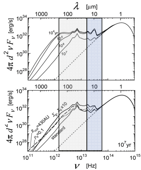
Figure 7: Predicted spectra of dust excesses from protoplanetary disks as a function of age -upper plot - and, for a given age disk, different dust size distributions and disk density profiles – lower plot 20 . The blue band shows the MIR coverage of JWST and the grey band the FIR coverage of SPICA
